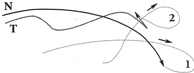
Figure 4-20b. Overlaid rod-tip pathways, including counterflex and rebound, along with subsequent loop shapes in two consecutive short-line casts. (N) Slightly convex pathway of the rod tip during a normally accelerated cast, resulting in a clean loop (1). (T) Deeply concave pathway of the rod tip during a cast where the rod is jerked forward, resulting in a tailing loop (2). Note that the tailing line must climb significantly upwards in order to unroll. Sequences from the video, The Fifteen Most Common Casting Errors .
