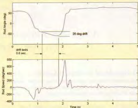
Figure 4. Rod drift is a powerful technique that can increase distance and efficiency. The upper half of Figure 4 shows how the expert's drift leads to a 20-degree increase in the casting arc over a 0.6-second time interval.
